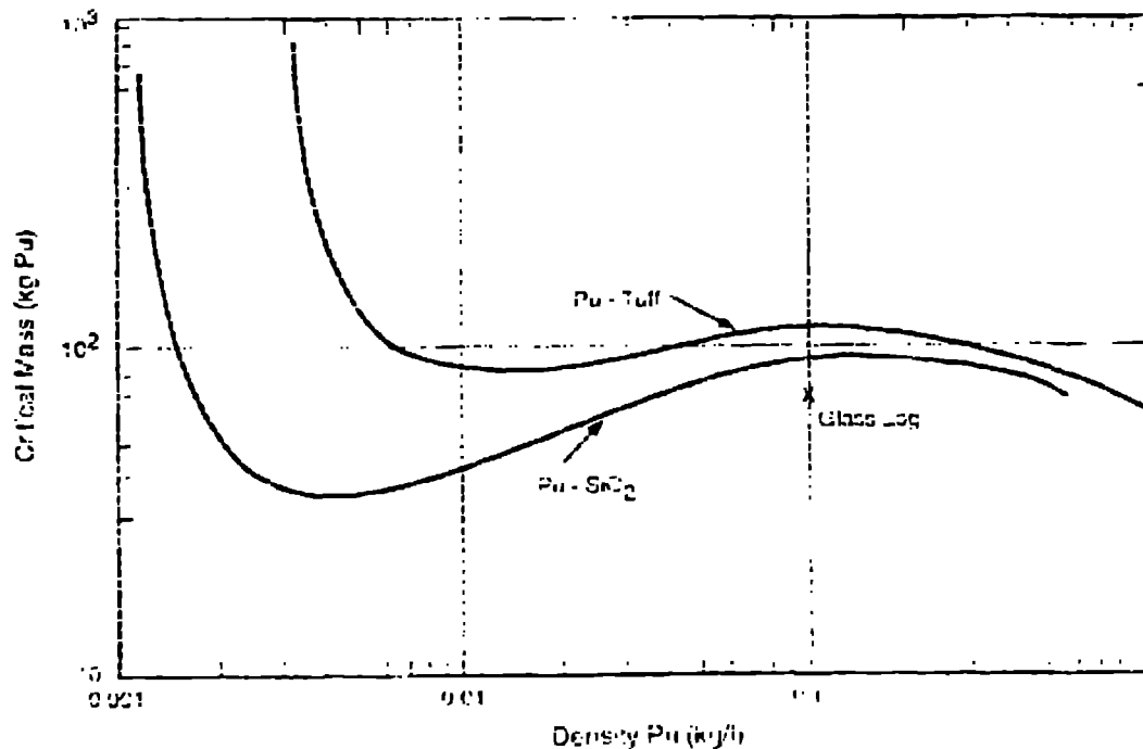
Figure 13. Reflected critical mass of plutonium metal mixed with tuff or SiO 2 vs. plutonium density (1000 temperature). This figure is analogous to Figs. 1 and 2. However, the function for Pu-tuff shows a much increased minimum critical mass (85 kg at 0.015 kg/l, compared to 35 kg at 0.004 kg/l); thus eliminating the need to consider the dry criticality as postulated in Ref. 1. The increased value of the minimum critical density asymptote should be noticed.
